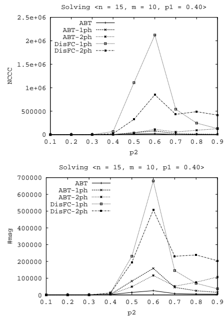
Figure 7. Number of non concurrent constraints checks (top) and exchanged messages (bottom) performed by ABT, ABT-1ph, ABT-2ph, DisFC-1ph and DisFC-2ph when solving PKC DisCSPs with p_1 = 0.4 .
