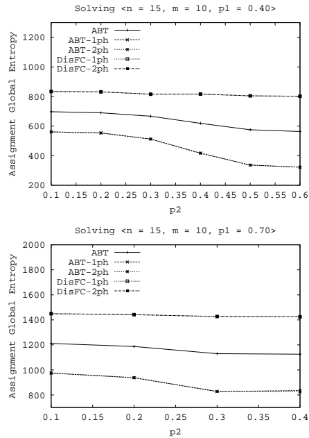
Figure 9. Assignment privacy in terms of entropy for ABT, ABT-2ph/1ph, DisFC-2ph/1ph for p_1 = 0.4 (left) and p_1 = 0.7 (right).
