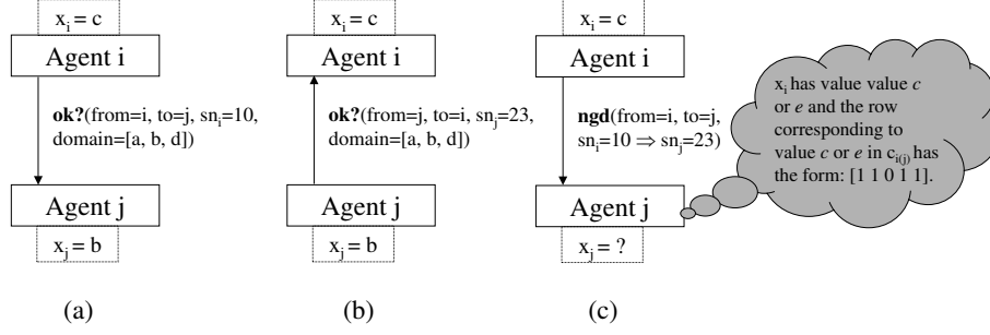
Figure 6. Information deduced by a DisFC-1ph agent after receiving a ngd message from a higher priority agent.
