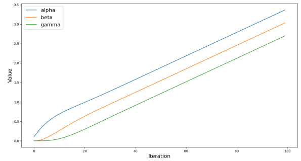
Figure 4: \alpha, \beta, \gamma as a function of the number of iterations, on a cycle with three function-nodes, with a damping factor \lambda = 0.9 .
