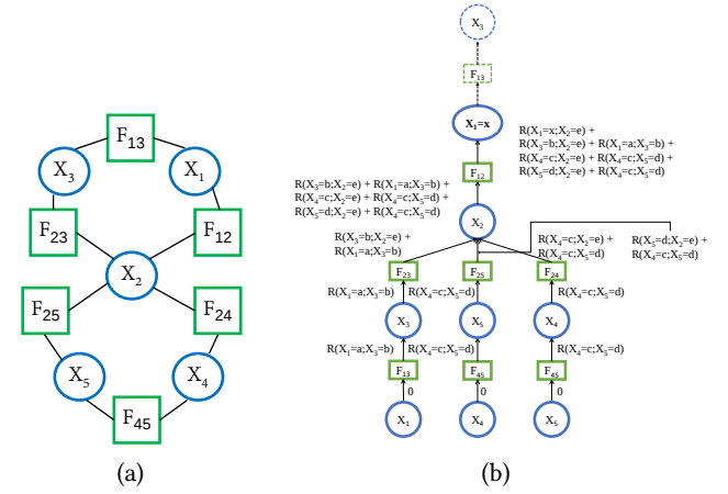
Figure 1: (a) A lemniscate factor-graph. (b) An example of a BCT for a belief in the message sent from X_1 to the function-node F_{13} at time t = 6 in the lemniscate depicted on the left.
