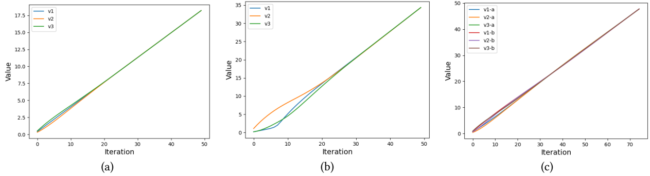
Figure 5: Sum of beliefs as a function of the number of iterations for (a) three value assignments of a three function-node cycle with a consistent minimal route and immediate convergence; (b) three value assignments of a three function-node graph with a consistent minimal route, but with a tail (not immediate convergence); (c) Variable assignment of six values in a three function-node cycle graph – an inconsistent minimal route – and with no tail.
