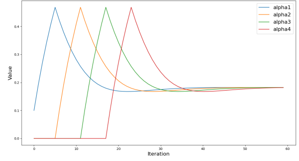
Figure 3: \alpha_1, \alpha_2, \alpha_3, \alpha_4 as a function of the number of iterations, on a cycle with three function-nodes, with a damping factor \lambda = 0.9 .
