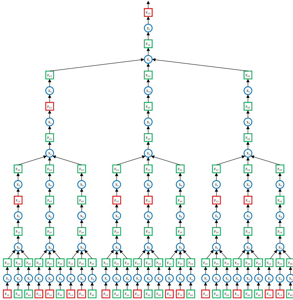
Figure 7: BCT of a leminscate factor graph with three function nodes in each cycle
