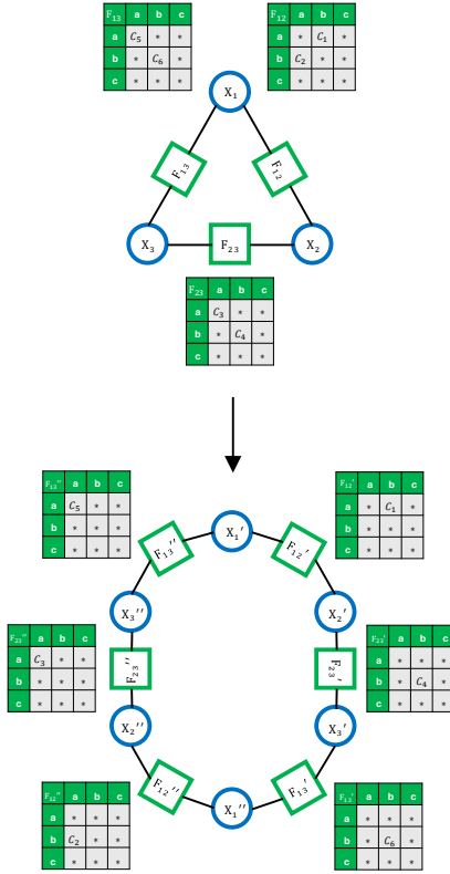
Figure 6: Inconsistent route in a single-cycle graph example
