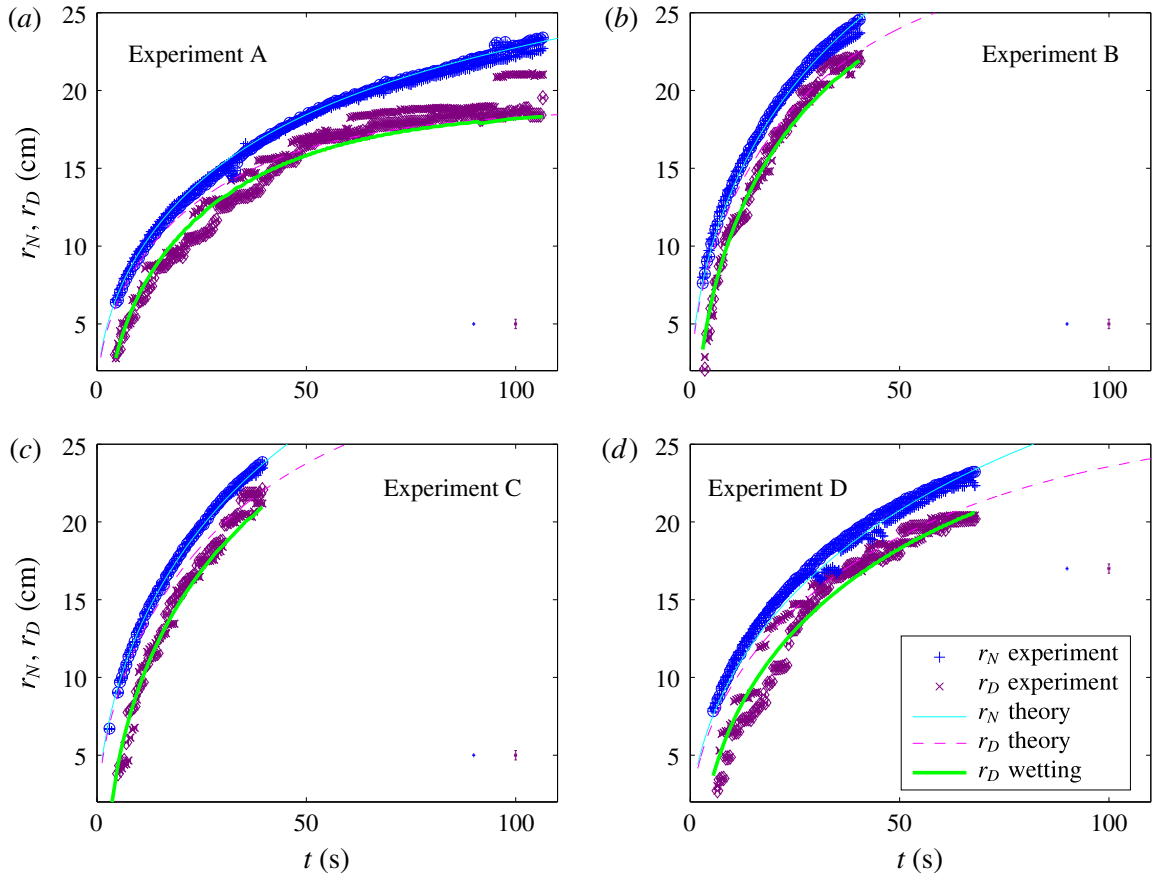
FIGURE 10. (Colour online) Experimental measurements and theoretical predictions of r_N ( \circ , + ) and r_D ( \diamond , \times ) for gravity currents with parameters given in table 1, where the two symbols denote the left and the right fronts (see figure 9a) respectively. Error bars for r_N and r_D are shown on the bottom right corner in corresponding colour. The theoretical predictions are marked with — (cyan) and ---- (magenta) for the fluid and drainage fronts. A correction to the early-time evolution of the drainage owing to finite-time wetting of the substrate is marked with — (green).
