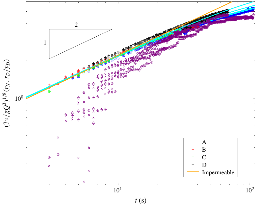
FIGURE 11. (Colour online) Measurements of the fronts r_N (+, o, blue, red, green and black) and r_D (◇, ×), where the two symbols denote the left and the right fronts, of gravity currents with parameters given in table 1, normalized with respect to the early time solutions (2.14b) and (2.15a) respectively. The solution for a constant-flux gravity current on an impermeable surface (— orange) is shown for reference, and the theoretical predictions for the fluid front r_N are shown (— cyan).
