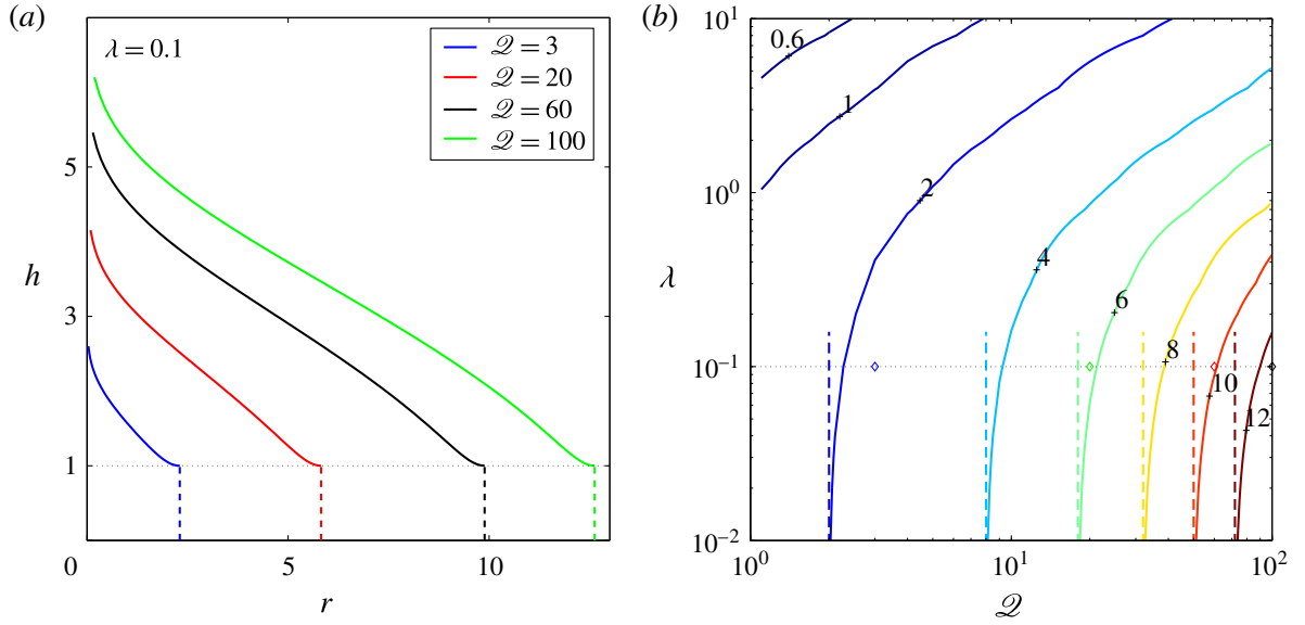
FIGURE 5. (Colour online) Numerical solutions to the steady-state boundary-value problem in the draining region (2.16). (a) Steady-state solutions of the free surface for \lambda = 0.1 and for \mathcal{Q} = 3, 20, 60, 100 , where dash lines mark the position of the drainage front in each case. (b) Contours of the steady-state position of the drainage front r_D as a function of \mathcal{Q} and \lambda (solid curves, contour value marked by adjacent numbers). In the limit \lambda \ll 1 the solution approaches r_D = \sqrt{2\mathcal{Q}} (vertical dash lines). The \diamond shapes along the \lambda = 0.1 grid line represent the points in the phase space that correspond to the solutions shown in (a). In all cases we assume that \mathcal{Q}_D = 0 .
