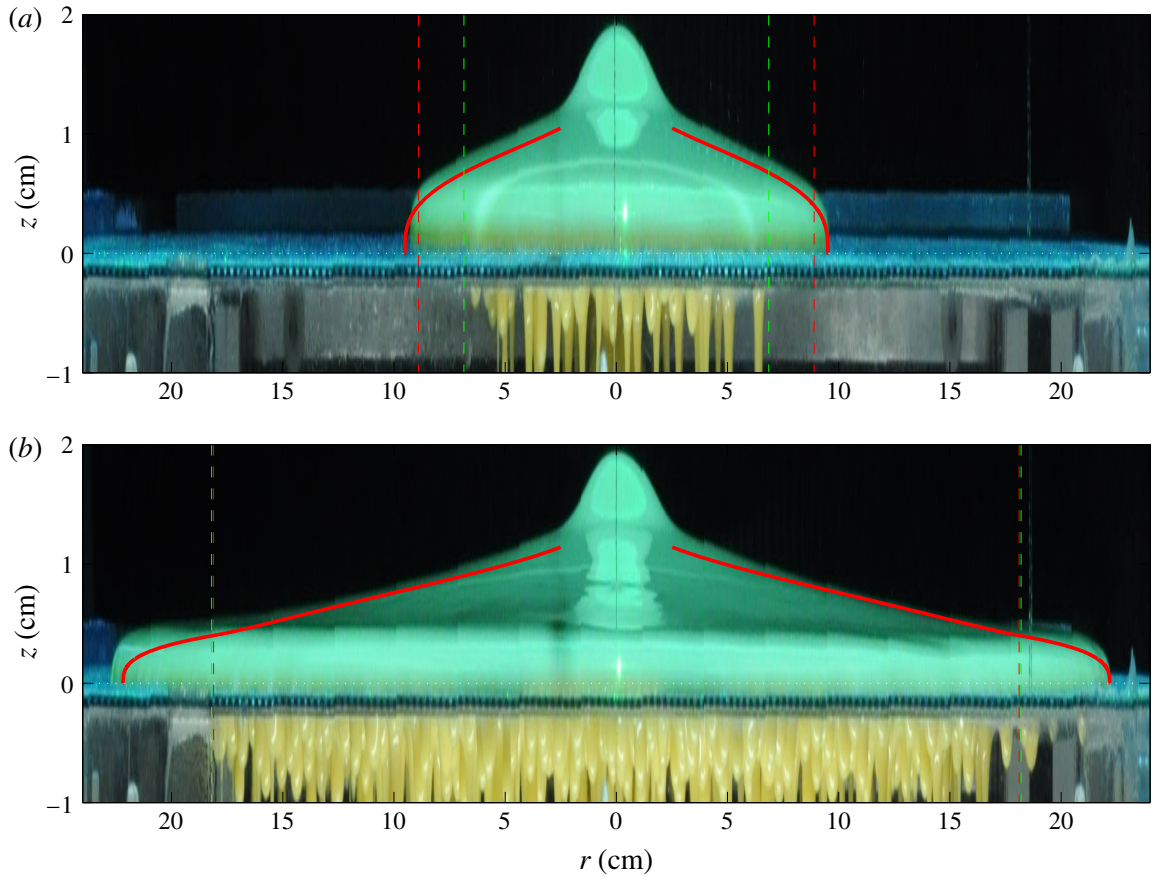
FIGURE 12. (Colour online) Snapshots from side view from experiment A (table 1) at t=10 s (a) and at t=100 s (b). The theoretical prediction of h is shown (—) and the corresponding predictions of the drainage fronts are shown in ---- (red) for the wetting-excluded theory and in ---- (green) for the delayed-wetting correction. The position z=0 is the top surface of the substrate at the centre (---- yellow).
