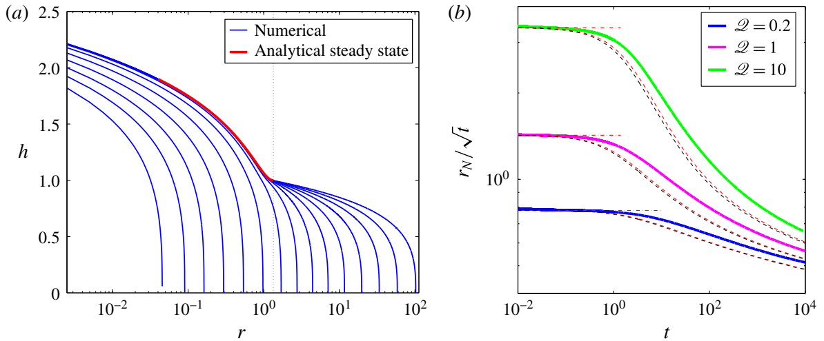
FIGURE 2. (Colour online) (a) Numerical solution of the evolution of the current for \lambda = 0.1 , \mathcal{Q} = 1 , showing the evolution of the free surface (— blue) starting at t = 10^{-2} and ending at t = 3.8 \times 10^4 . The temporal spreading of the profiles is uniform in the \log(t) space. The steady-state solution of the drainage-active region in the limit \mathcal{Q}_D = 0 (2.17) is shown (— red), where the position of the steady-state drainage front is marked by a vertical grid line. (b) Evolution of the fluid front r_N for \lambda = 0.1 and for \mathcal{Q} = 0.2, 1, 10 , showing the full numerical solutions (thick curves), the asymptotic estimates of the early time evolution (----, red), and the asymptotic estimates of the late-time evolution (---- red) for the case \lambda \ll 1 and \mathcal{Q} = 0 and (---- black) for the finite \lambda and non-zero \mathcal{Q}_D case, which are evaluated also at early time.
