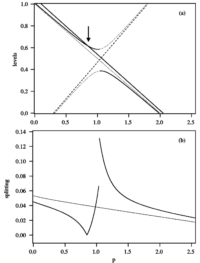
FIG. 1. Sketch of the typical behavior of the energy levels of a classically chaotic quantum system as the parameter p is changed. In (a) the two solid thick lines describe a couple of quasidegenerate levels of different symmetry. The thin dotted line represents the lower level of the tunneling doublet in the unperturbed case. The dashed line describes a colliding third level. In (b) we show the splitting of the two quasidegenerate levels in the perturbed and unperturbed case (thin dotted line). All the units are arbitrary.
