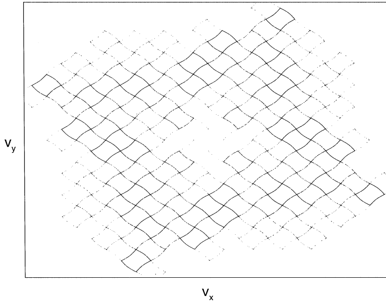
FIGURE 1 A typical relativistic stochastic web.
