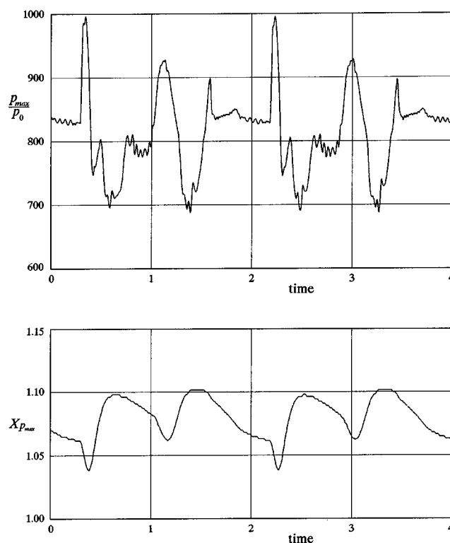
FIG. 6. Time variation of the maximum pressure along the wedge surface (top plot) and its location (bottom plot).
