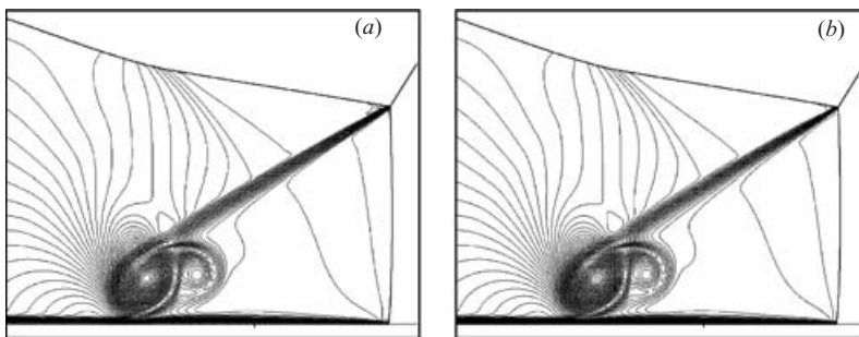
FIGURE 12. Isopycnics for the self-similar viscous flow model, calculated on two different grids, for M_i = 3.22 , \theta_w = 32^\circ and Re = 4000 . (a) 500 \times 150 grid; (b) 1000 \times 300 grid. The density contour increment is \Delta\rho/\rho_0 = 0.07 .
