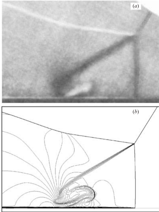
FIGURE 11. Comparison between an experiment (a), and the corresponding numerical simulation (b), for the non-stationary viscous flow. The incident shock wave Mach number is M_i = 3.22 , the wedge angle is \theta_w = 32^\circ . The instantaneous Reynolds number is Re = 12\,500 .
