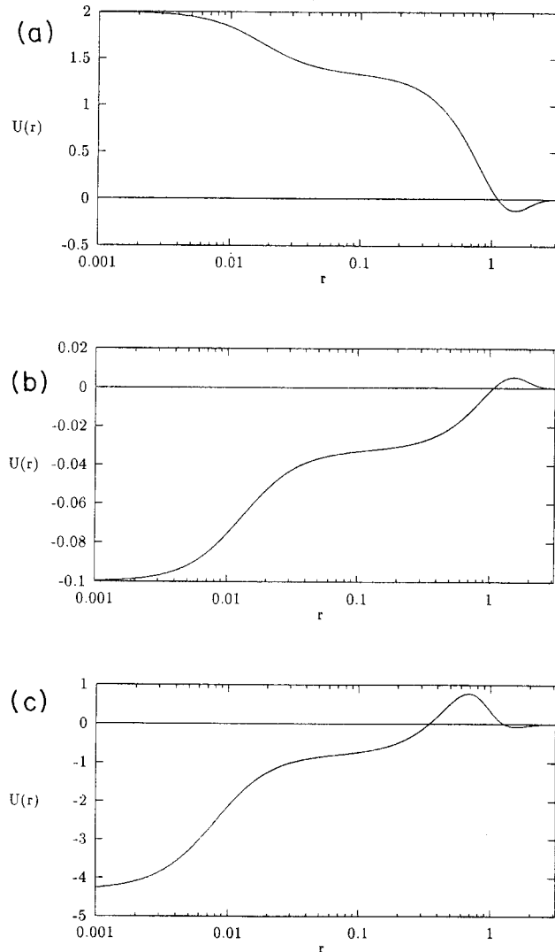
FIG. 2. Distribution of potential U(r) for Pe = 10^4 and different values of \varepsilon and \alpha : (a) \varepsilon = 0 ; (b) \varepsilon = 0.35 , \alpha = 1 ; (c) \varepsilon = 0.35 , \alpha = 4 .
