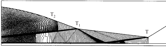
FIGURE 16. Self-similar Mach number contours for the case shown in figure 15(d) as calculated using a mesh refinement with a weak shocks emanating from T_1 .
