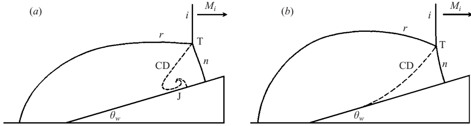
FIGURE 1. (a) The jetting and (b) no-jetting effects in SMR. i , incident shock wave; r , reflected shock wave; n , Mach shock (here called the n -shock); CD, contact discontinuity; T, triple point (Mach node); J, jet.
