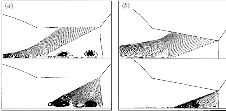
FIGURE 14. Streamlines in strong and weak jetting for M_i = 5 : (a) strong jetting for \theta_w = 40^\circ ; (b) weak jetting for \theta_w = 55.15^\circ
