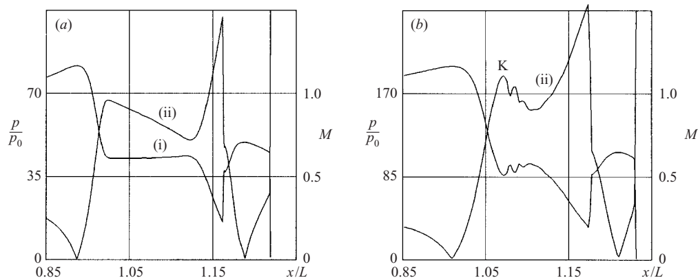
FIGURE 21. Pressure (i) and self-similar Mach number (ii) distributions along the wall in the jet region for self-similar flows. (a) M_i = 4.5 , \theta_w = 36^\circ and \gamma = 1.4 ; (b) M_i = 7 , \theta_w = 30^\circ and \gamma = 1.3 .
