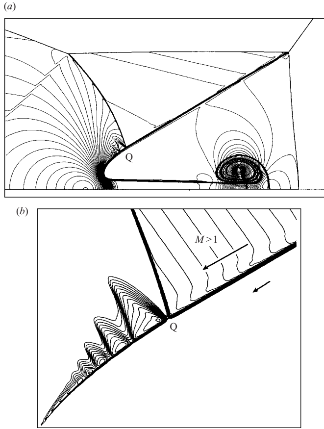
FIGURE 22. Cascade interaction along the contact discontinuity. Adaptive mesh refinement for figure 18(d). (a) Isopycnics of the forced stable flow. (b) Supersonic Mach number contours near the interaction of the n_1 -shock and the contact discontinuity.
