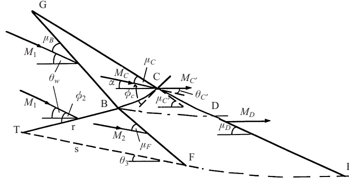
FIGURE 3. Enlargement of a section of the schematic drawing shown in figure 2 and definition of relevant parameters.
