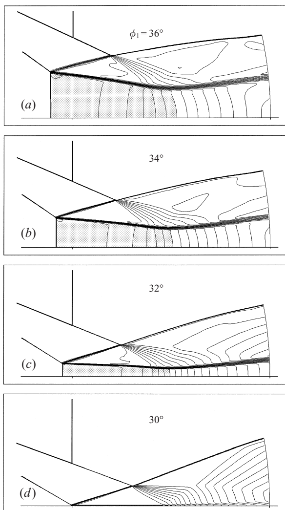
FIGURE 11. Numerical calculations of the flow Mach number contours of the wave configurations for M_0 = 4.96 , p_w = p_1 and four different values of incident shock wave angle, \phi_1 .
