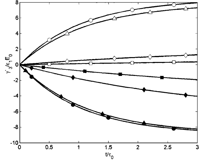
FIG. 7. Time dependence of a free charge \gamma'_3 at location \vec{N} = (0, 0, 1) in a constant external electric field \vec{E}_0 . Vector \vec{E}_0 is located in the plane \vec{e}_1, \vec{e}_3 ( \vec{E}_0 \cdot \vec{e}_2 = 0 ) and is directed by the angle \theta = \pi/4 with the axis of symmetry of the spheroid ( \circ : a'_1 = a'_2 = 0.05 , \kappa_e/\kappa_\sigma = 0.1 , prolate spheroid; \square : a'_1 = a'_2 = 50 , \kappa_e/\kappa_\sigma = 0.1 , oblate spheroid; \diamond : a'_1 = a'_2 = 1 , \kappa_e/\kappa_\sigma = 0.1 , sphere; \triangle : a'_1 = 50 , a'_2 = 0.05 , \kappa_e/\kappa_\sigma = 0.1 , ellipsoid; \bullet : a'_1 = a'_2 = 0.05 , \kappa_e/\kappa_\sigma = 10 , prolate spheroid; \blacksquare : a'_1 = a'_2 = 50 , \kappa_e/\kappa_\sigma = 10 , oblate spheroid; \blacklozenge : a'_1 = a'_2 = 1 , \kappa_e/\kappa_\sigma = 10 , sphere; \blacktriangle : a'_1 = 50 , a'_2 = 0.05 , \kappa_e/\kappa_\sigma = 10 , ellipsoid).
