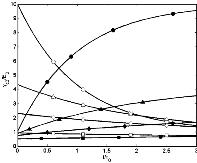
FIG. 5. Time dependence of a surface charge \gamma_{c3} at location \vec{N} = (0, 0, 1) in a constant external electric field \vec{E}_0 . Vector \vec{E}_0 is located in the plane \vec{e}_1, \vec{e}_3 ( \vec{E}_0 \cdot \vec{e}_2 = 0 ) and is directed by the angle \theta = \pi/4 with the axis of symmetry of the spheroid ( \circ : a'_1 = a'_2 = 0.05 , \kappa_e/\kappa_\sigma = 0.1 , prolate spheroid; \square : a'_1 = a'_2 = 50 , \kappa_e/\kappa_\sigma = 0.1 , oblate spheroid; \diamond : a'_1 = a'_2 = 1 , \kappa_e/\kappa_\sigma = 0.1 , sphere; \triangle : a'_1 = 50 , a'_2 = 0.05 , \kappa_e/\kappa_\sigma = 0.1 , ellipsoid; \bullet : a'_1 = a'_2 = 0.05 , \kappa_e/\kappa_\sigma = 10 , prolate spheroid; \blacksquare : a'_1 = a'_2 = 50 , \kappa_e/\kappa_\sigma = 10 , oblate spheroid; \blacklozenge : a'_1 = a'_2 = 1 , \kappa_e/\kappa_\sigma = 10 , sphere; \blacktriangle : a'_1 = 50 , a'_2 = 0.05 , \kappa_e/\kappa_\sigma = 10 , ellipsoid).
