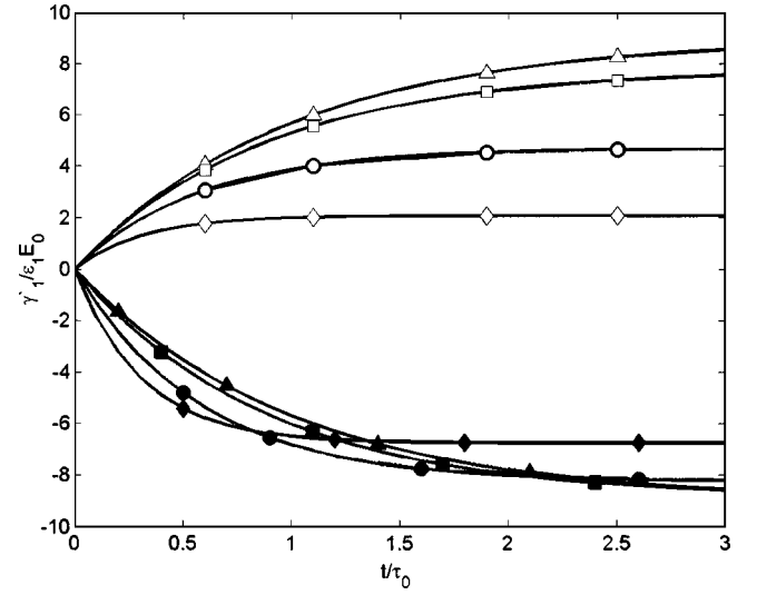
FIG. 6. Time dependence of a free charge \gamma'_1 at location \vec{N} = (1, 0, 0) in a constant external electric field \vec{E}_0 . Vector \vec{E}_0 is located in the plane \vec{e}_1, \vec{e}_3 ( \vec{E}_0 \cdot \vec{e}_2 = 0 ) and is directed by the angle \theta = \pi/4 with the axis of symmetry of the spheroid ( \circ : a'_1 = a'_2 = 0.05 , \kappa_e/\kappa_\sigma = 0.1 , prolate spheroid; \square : a'_1 = a'_2 = 50 , \kappa_e/\kappa_\sigma = 0.1 , oblate spheroid; \diamond : a'_1 = a'_2 = 1 , \kappa_e/\kappa_\sigma = 0.1 , sphere; \triangle : a'_1 = 50 , a'_2 = 0.05 , \kappa_e/\kappa_\sigma = 0.1 , ellipsoid; \bullet : a'_1 = a'_2 = 0.05 , \kappa_e/\kappa_\sigma = 10 , prolate spheroid; \blacksquare : a'_1 = a'_2 = 50 , \kappa_e/\kappa_\sigma = 10 , oblate spheroid; \blacklozenge : a'_1 = a'_2 = 1 , \kappa_e/\kappa_\sigma = 10 , sphere; \blacktriangle : a'_1 = 50 , a'_2 = 0.05 , \kappa_e/\kappa_\sigma = 10 , ellipsoid).
