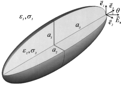
FIG. 1. Ellipsoid with semi-axes a_1, a_2, a_3 ( a_1 = a_2 < a_3 : prolate spheroid; a_1 = a_2 > a_3 : oblate spheroid) and electric permittivity \epsilon_2 and conductivity \sigma_2 inside a host medium with permittivity \epsilon_1 in the external electric field \vec{E}_0 .
