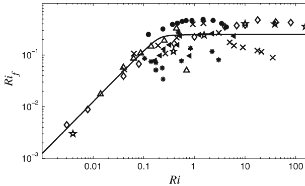
Fig. 4 Ri dependence of the flux Richardson number Ri_f = -\beta F_z/(\tau S) for meteorological observations: slanting black triangles (Kondo et al. 1978), snowflakes (Bertin et al. 1997); laboratory experiments: slanting crosses (Rehmann and Koseff 2004), diamonds (Ohya 2001), black circles (Strang and Fernando 2001); DNS: five-pointed stars (Stretch et al. 2001); LES: triangles (our DATABASE64). Solid line shows the steady-state EFB model, Eq. 56, with Ri_f \rightarrow R_\infty = 0.25 at Ri \rightarrow \infty
