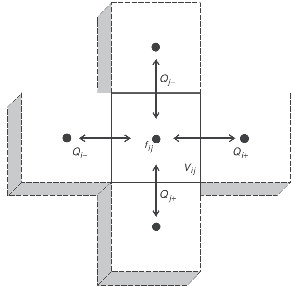
Figure 2 Quadratic finite volume in 2D
