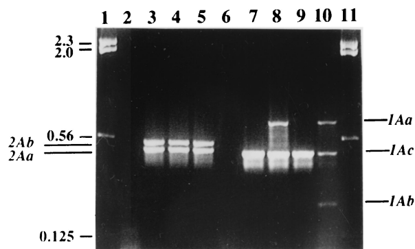
Fig. 4. Agarose gel (2.2%) electrophoresis of PCR products obtained with specific primers for cry1 and cry2 . Lanes 1 and 11, molecular weight markers ( \lambda_{DNA} cleaved by HindIII ), with sizes (in kb) indicated on left; lanes 2–5, respectively, DNA of (all amplified with a mixture of specific primers for cry2 ) B. thuringiensis subsp. kurstaki (melanin producing mutant Bt-m ), B. thuringiensis subsp. kurstaki (parent; Bt-01 ), B. thuringiensis subsp. kurstaki HD-73, and B. thuringiensis subsp. kurstaki HD-1; lanes 6–10 (all amplified with a mixture of specific primers for cry1 ), respectively, negative controls (without template), DNA of B. thuringiensis subsp. kurstaki (melanin producing mutant Bt-m ), Bt-01 (parent), B. thuringiensis subsp. kurstaki HD-73, and B. thuringiensis subsp. kurstaki HD-1.
