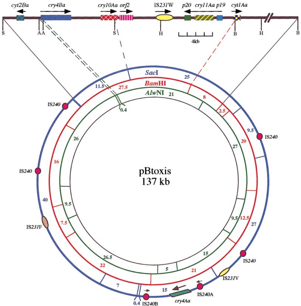
FIG. 3. Restriction map of the 137-kb B. thuringiensis subsp. israelensis pBtoxis plasmid. Numbers represent sizes of the relevant fragments of Bam HI (B), Sac I (S), and Alw NI (A). The region containing most of the known genes, of about 26 kb ( Sac I– Sac I– Bam HI– Hind III), is enlarged about 1.5-fold (see 4 kb bar). Genes are indicated by colored boxes and direction of transcription—by arrows. Insertion sequences are marked as circles (the IS240s) or oval bodies (IS231s).
