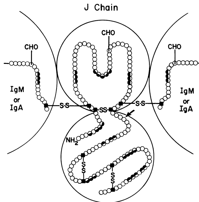
FIG. 4. A proposed two-domain structure for J chain. A model for the three-dimensional structure of mouse J chain is schematically represented by using half-closed circles to indicate stretches of hydrophobic amino acid residues, closed boxes to denote cystine residues, and open circles to represent all the remaining amino acid residues. The arrow indicates a peptide bond hypersensitive to cleavage by subtilisin. Also depicted are the carboxyl-terminal IgM or IgA domain and the 19-residue secreted tails to which the J chain is disulfide-bonded. See text for more detailed explanation.
