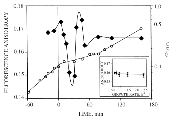
Fig. 7. DPH fluorescence anisotropy (◆) and culture biomass (○) during a nutritional shift-down (at time zero) to \alpha MG/glucose = 10. The culture was diluted 1:2 by a fresh, prewarmed medium with the same \alpha MG/glucose ratio at 60 min. The line drawn through anisotropy values is an interpolation fitting. Inset: DPH fluorescence anisotropy as a function of E. coli B/r steady-state growth rate, varied by \alpha MG/glucose ratio (0, 5, 10 and 20) or the addition of casein hydrolysate (1%) to glucose minimal medium.
