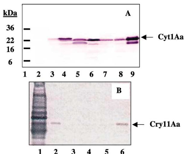
Fig. 2. Western blots of transgenic Anabaena and E. coli expressing CytGAa (A) and Cry11Aa (B) using anti-Cyt1Aa and antiserum against whole crystals, respectively. A: Lane 1, molecular size marker; lane 2, Anabaena PCC 7120 as a control; lane 3, pRVE4-C; lane 4, pRM4-C; lane 5, pRVE4-RC; lane 6, pRM4-RC; lane 7, pRVE4-ADRC; lane 8, pVE4-ADRC; lane 9, B. thuringiensis subsp. israelensis . B: Lane 1, B. thuringiensis subsp. israelensis ; lane 2, pSBJ2; lane 3, Anabaena PCC 7120 as a control; lane 4, pRVE4-C; lane 5, pRVE4-RC; lane 6, pRVE4-ADRC.
